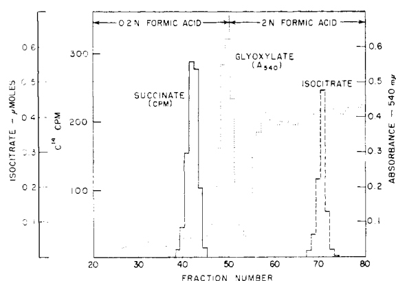
FIGURE 1: Chromatographic separation of acids. Isocitrate, glyoxylate, and succinate-2,3- ^{14}\text{C} were placed on a 10 by 80 mm column and eluted by the sequential addition of 100 ml of water, 150 ml of 0.2 N formic acid, and 150 ml of 2 N formic acid. Succinate was identified by placing 0.5-ml aliquots from each 5-ml fraction on planchets, drying, and measuring radioactivity with a gas flow counter. Another 0.5-ml aliquot was treated with dinitrophenylhydrazine for the detection of glyoxylate by the procedure of Friedemann and Haugen (1943) as modified by Smith and Gunsalus (1957). This reagent gave an absorbance of 0.042 and 0.416 for 0.5-ml samples of the eluting solvents, 0.2 N formic acid and 2 N formic acid, respectively. Isocitrate was determined by assaying a 0.5-ml aliquot by the method of Ochoa (1952). The first 20 fractions (water wash) did not contain significant levels of radioactivity or absorbing materials and are not shown on the figure. The ordinate scales refer to 0.5 ml.
