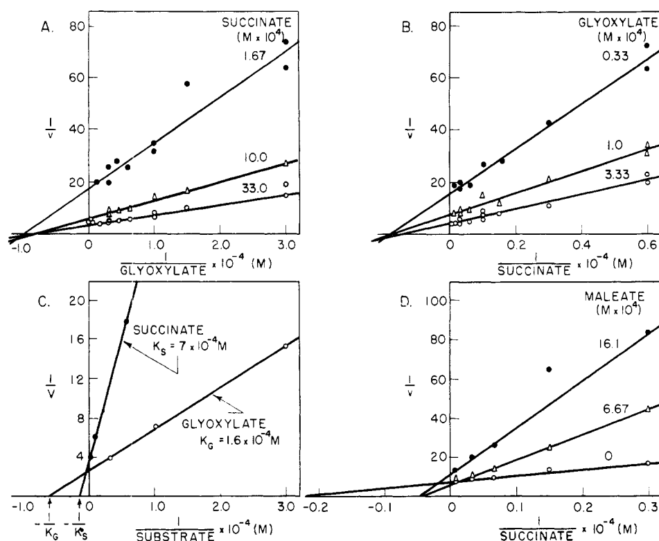
FIGURE 2: Reaction rate of isocitrate lyase, effect of substrate and inhibitor (maleate) concentration. Rates were measured as described in Methods. A 3-ml quartz cuvet (1-cm light path) contained in \mu moles: Tris buffer, pH 8.0, 200; \text{MnCl}_2 , 2; \text{MgCl}_2 , 6; cysteine hydrochloride (not neutralized), 4; NADP, 0.54; isocitrate dehydrogenase, 0.55 unit; isocitrate lyase (specific activity = 5), 0.97 unit; succinate, glyoxylate, and maleate, as shown.
